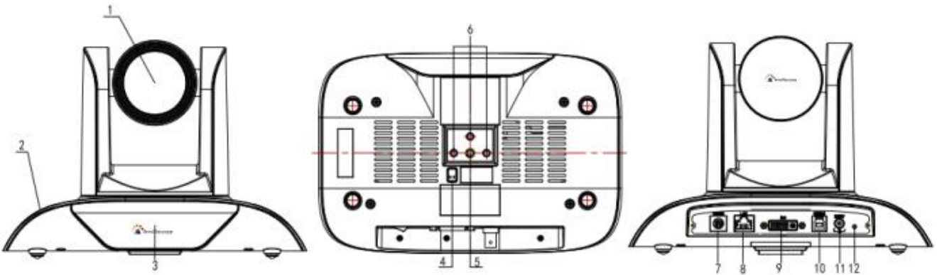
Figure 1.2. Interface of U3 (USB3.0) series
