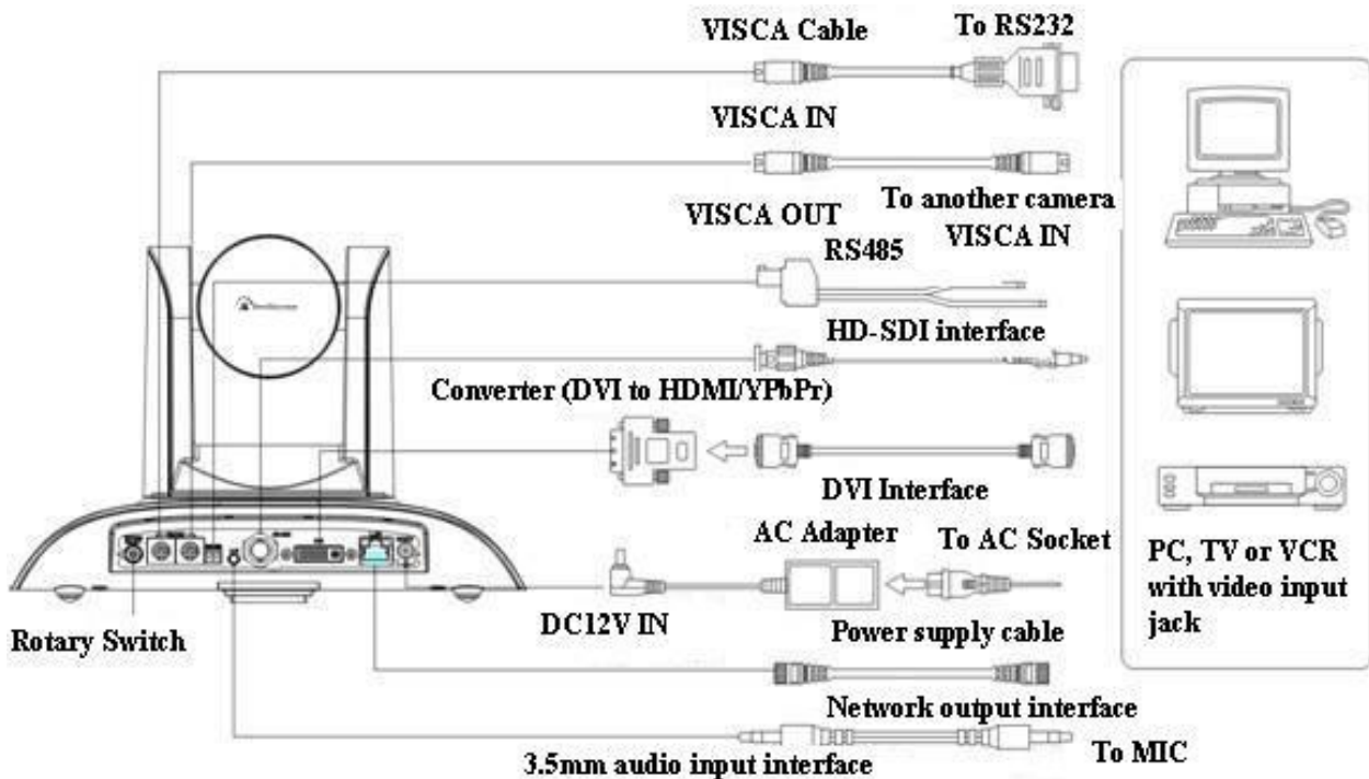
Figure 2.3 ST model external interface diagram
