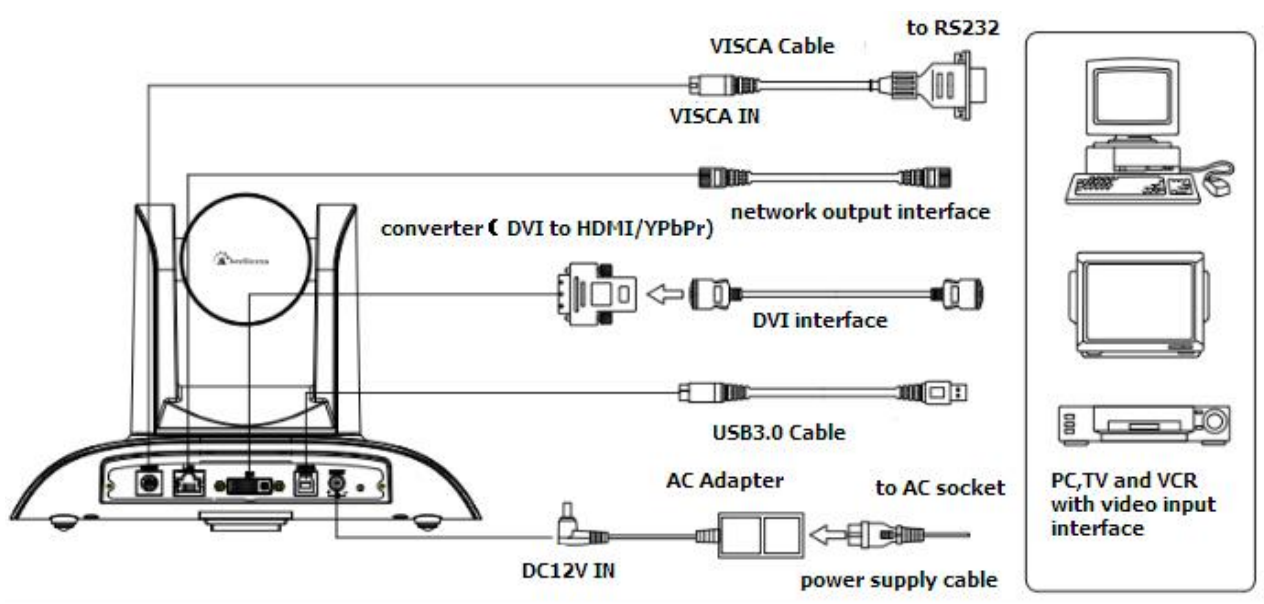
Figure 2.4 U3 model external interface diagram
