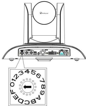
Figure 2.6 Rotary Dial diagram
