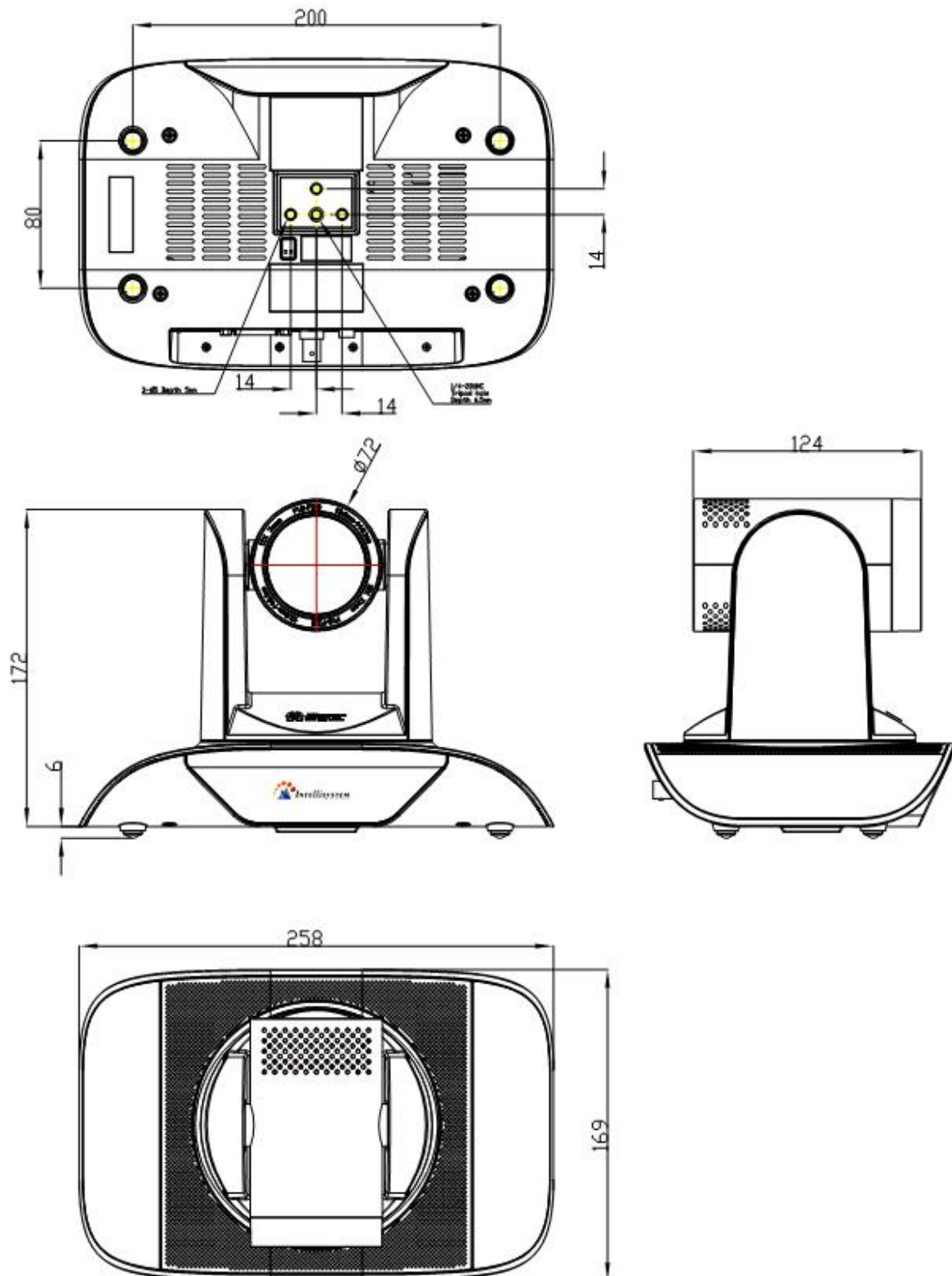
Figure 2.2 Camera dimension
