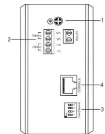
Bottom Panel
