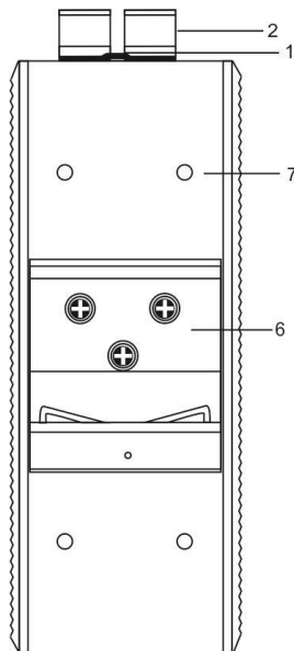
Rear panel
