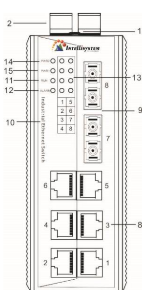
Front panel
