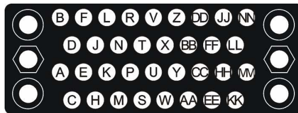
Distribution diagram of guiding feet on M34 cored jack
