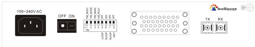
Rear Panel of IT-7304-PC/AC
