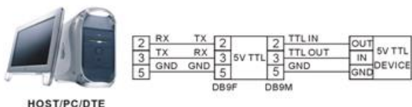
Connecting the RS232 port to a 5V TTL Device
