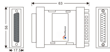
DB25M (Male/needle)
