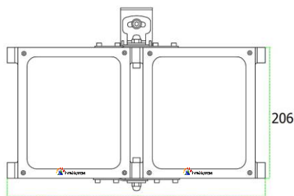
409 Front view
