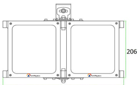
409 Front view
