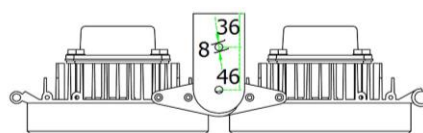
Vertical view
