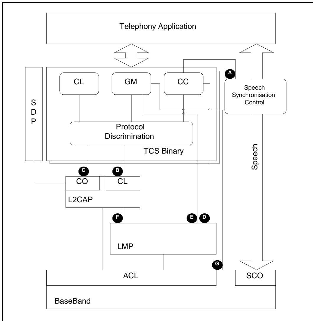
Figure 2.1: Protocol model
