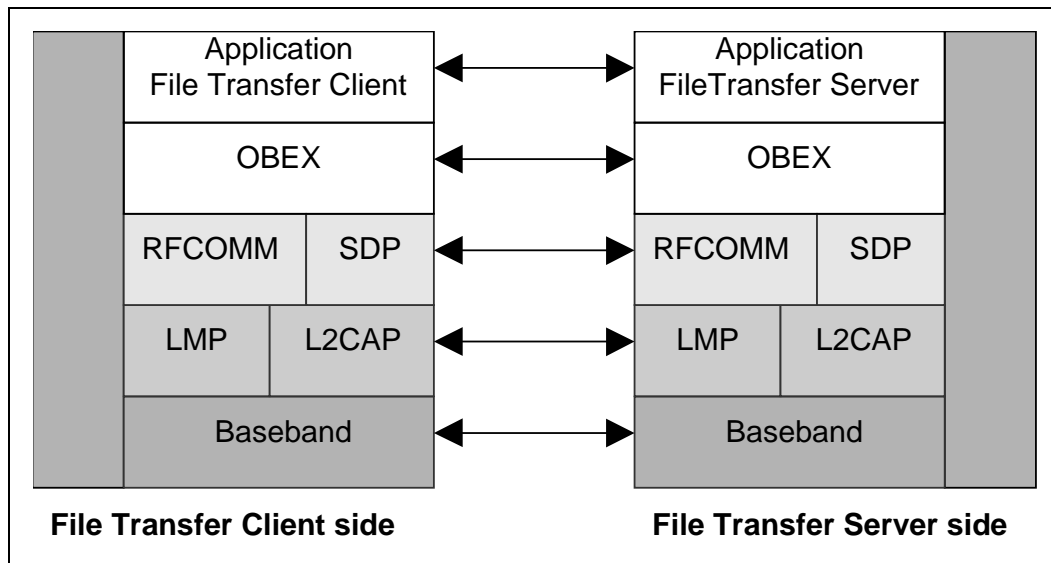
Figure 2.1: Protocol model
