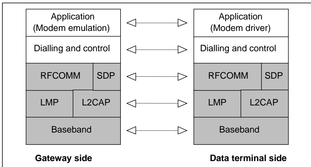
Figure 2.1: Protocol model
