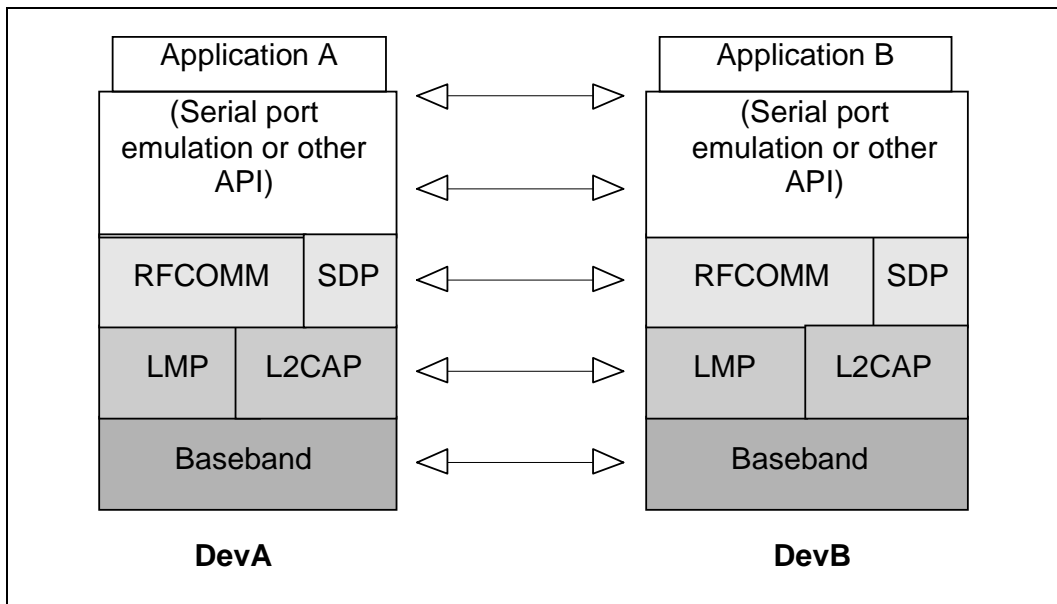
Figure 2.1: Protocol model
