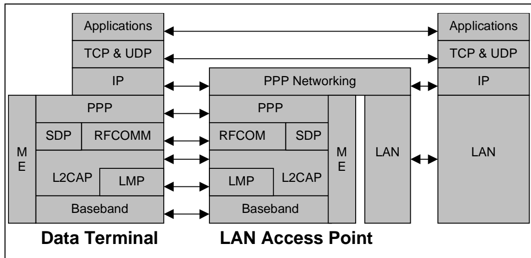
Figure 2.1: Protocol Stack
