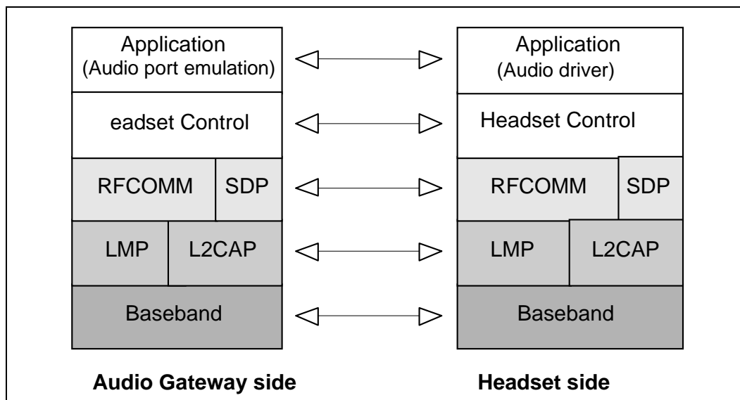
Figure 2.1: Protocol model
