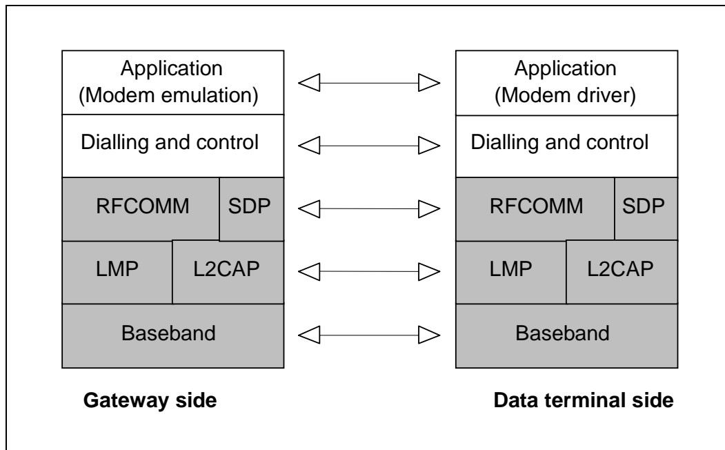
Figure 2.1: Protocol model
