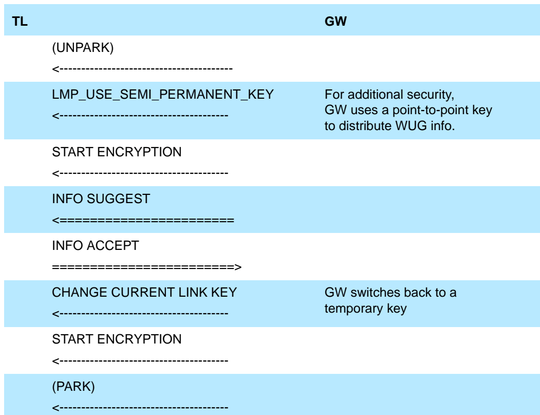
Figure 10.9: Signalling diagram for Configuration distribution
