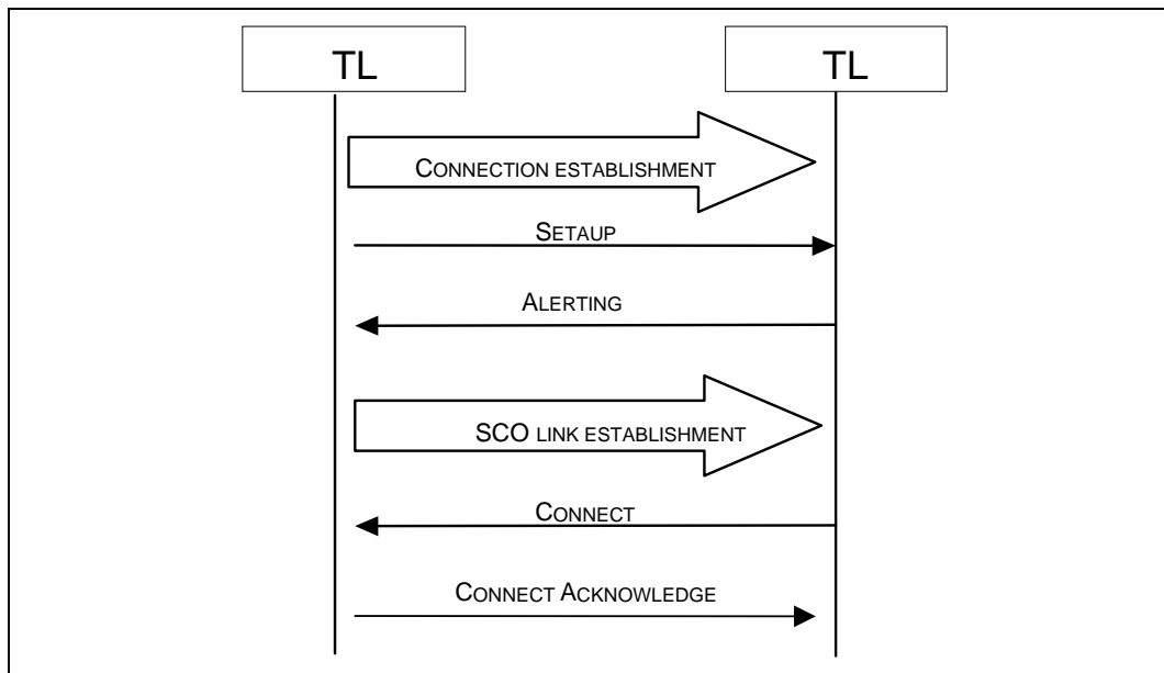
Figure 10.1: Call establishment
