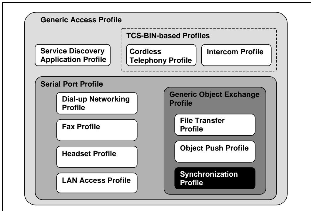
Figure 1.1: Bluetooth Profiles
